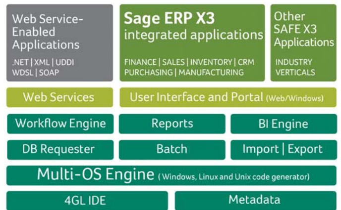
The Sage Application Framework for the Enterprise (SAFE X3): An open design
